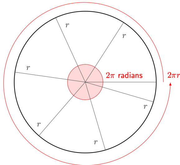
Figure 4: A circle divided by sectors with arc length equal to the radius.
