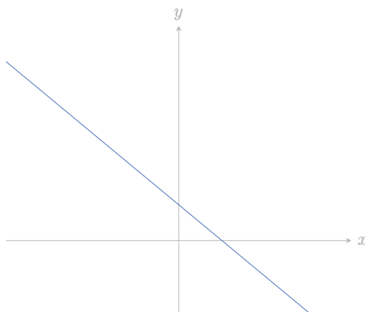
Figure 1: The line x + y = 1 plotted on an axis.
